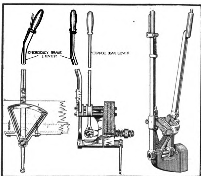
Fig. 15—Franklin Brakes and Change Gear Control.
